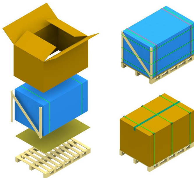
New packaging box with protection frame (modules will be protected by "N" shape plywood frame with soft EPE buffer layer, which will give horizontal support for shipment jolting )
