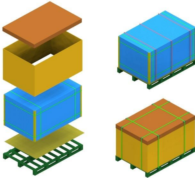
Current Packaging (module corners were protected by corrugated paper, no horizontal support)
